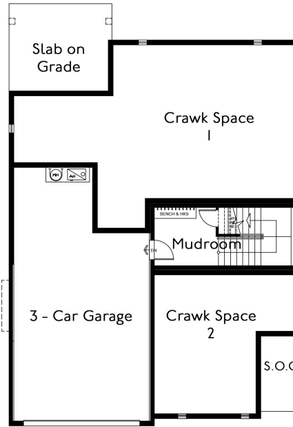
Basement Level
